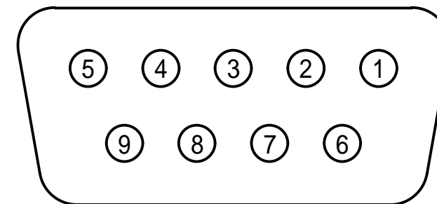
D-sub 9P FEMALE (TOP VIEW)
